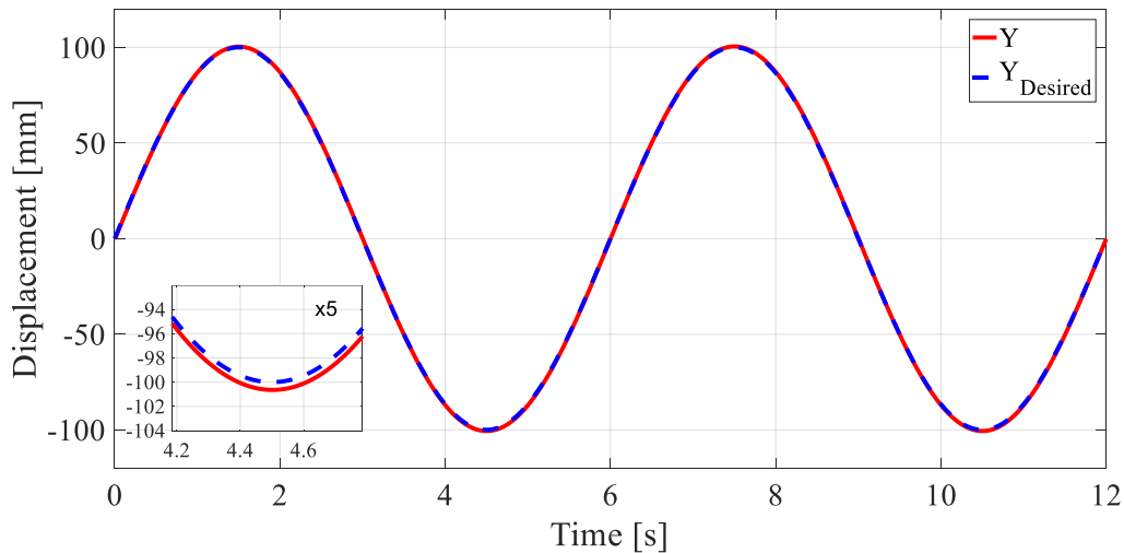
Fig.4. Compared position results for Y motion
