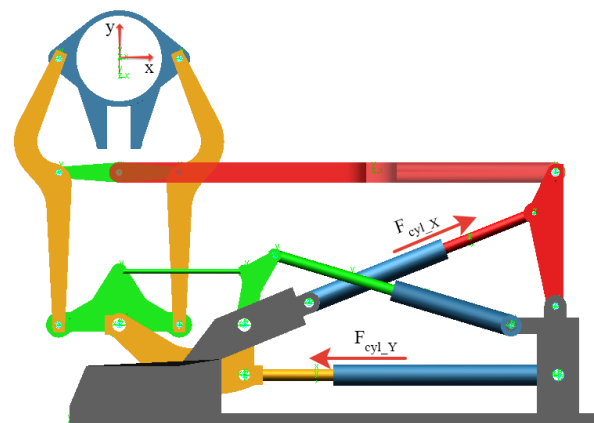
Fig.1. Multi-body model of the multi-DOF road simulator
